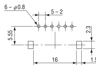
Mounting hole dimension (Tolerance : 0.1) (Board thickness t = 1.6)
