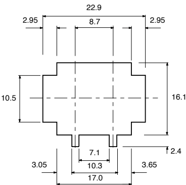
4P PANEL HOLE DIMENSION
