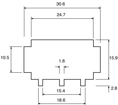
6P PANEL HOLE DIMENSION
