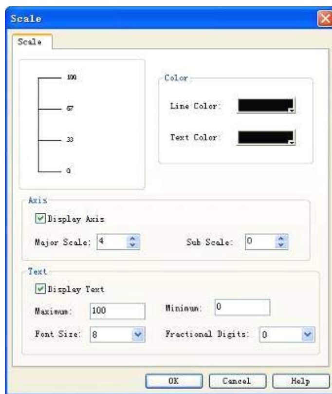
Figure 4-47: Scale dialog
