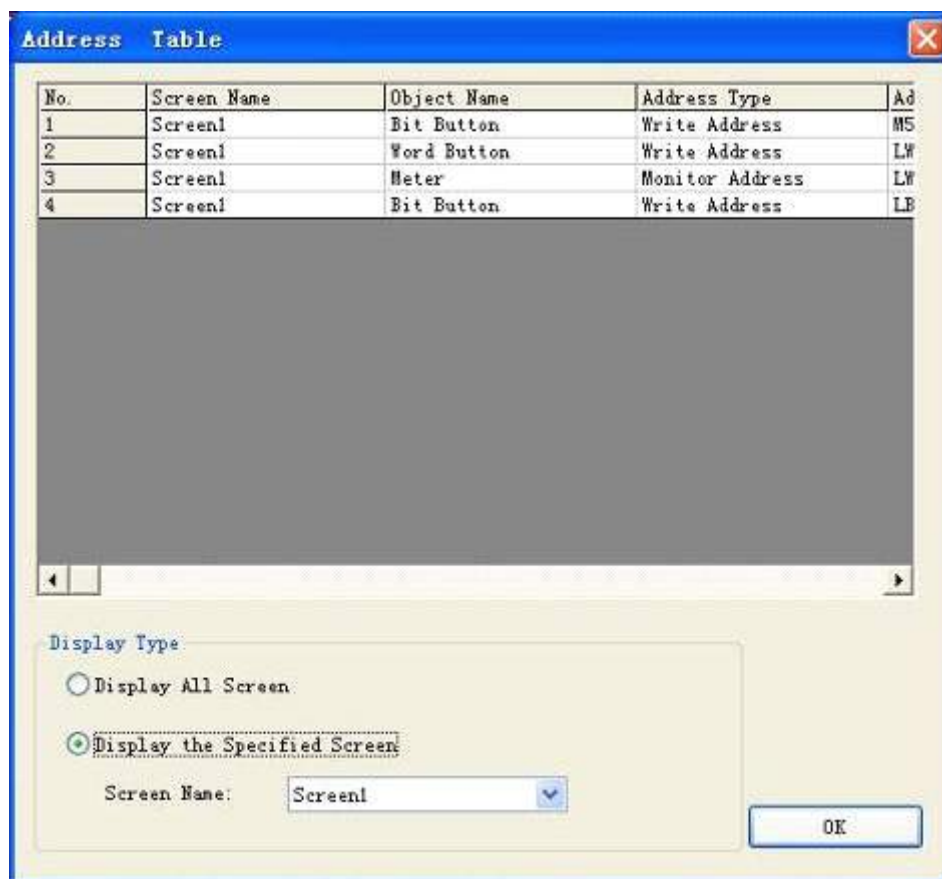
Figure 4-117: Address table
