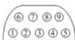
9DIND male configuration
