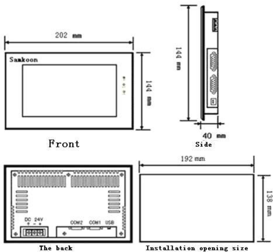
Figure 1-9: Installing dimensions of SA-5.7D/SA-5.7E/SA-5.7F
