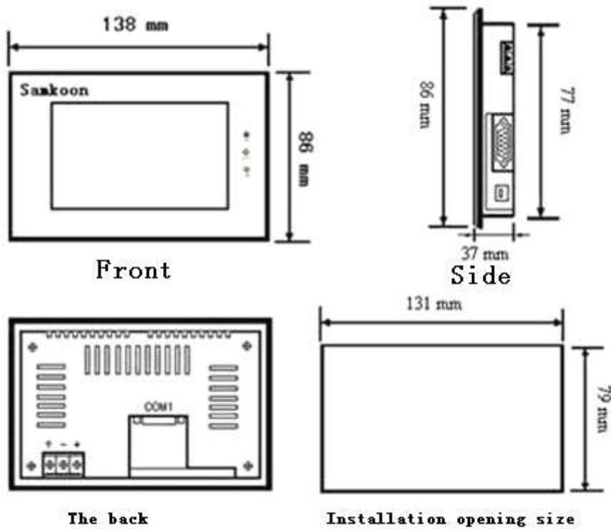
Figure 1-5: Installing dimensions of SA-4.3
