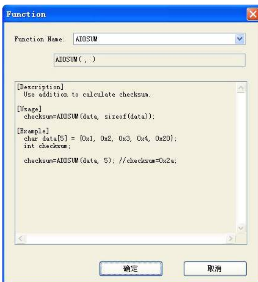
Figure 5-6 (Function Selection)
