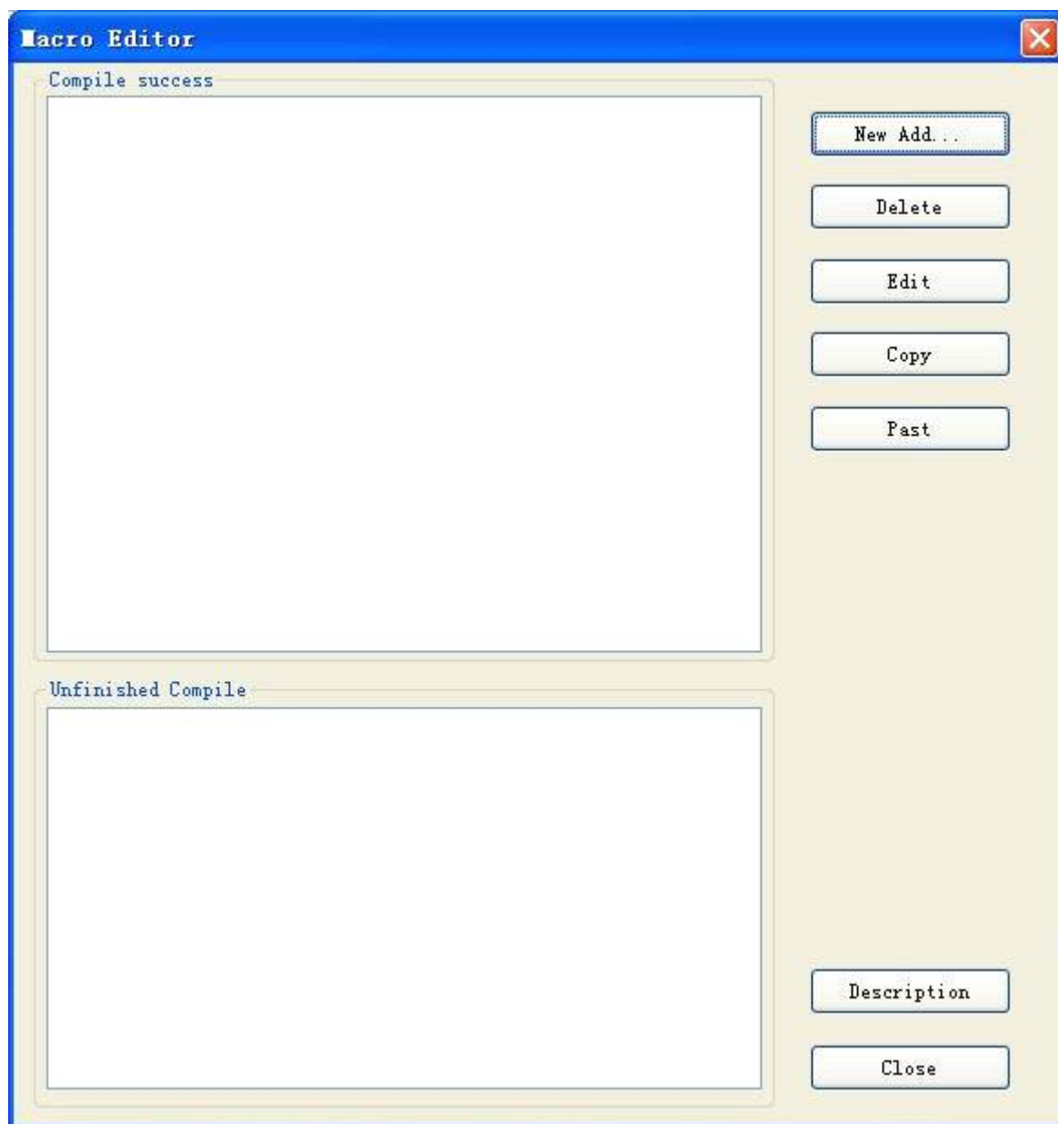
Figure 5-7 (Macro Editor)
