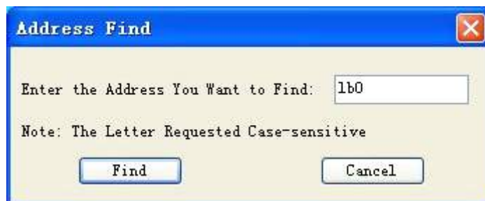
Figure 4-115: Address find
