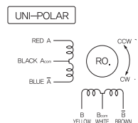
Wiring Diagram
