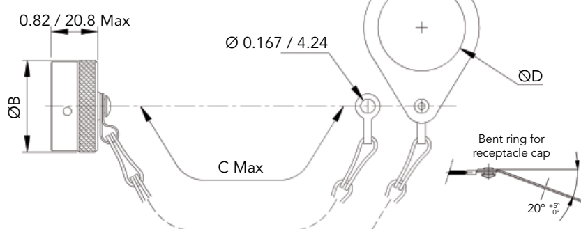
Cap for receptacle Type 502
