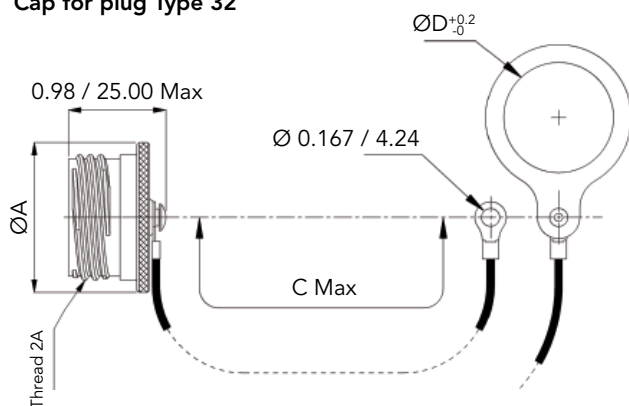
Cap for plug Type 32
